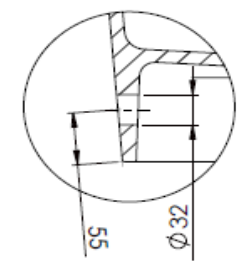
D (1:5)
